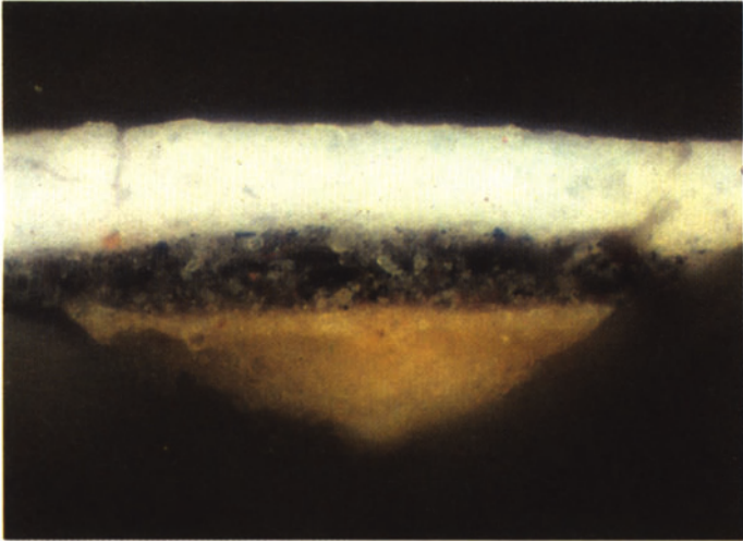
Fig. 8. Cross section ( 335\times ) from the top part of the white sash of the figure on the extreme left in no. A 6, showing from bottom to top: 1. the chalk and glue ground, 2. a thin layer of yellowish 'primuersel' (containing white lead and some brown pigment), 3. a dark mixture used for the underpainting (containing a translucent brown pigment, organic red pigment, white lead and possibly some chalk, black pigment and some red, either vermilion or red ochre), 4. a layer of white lead
